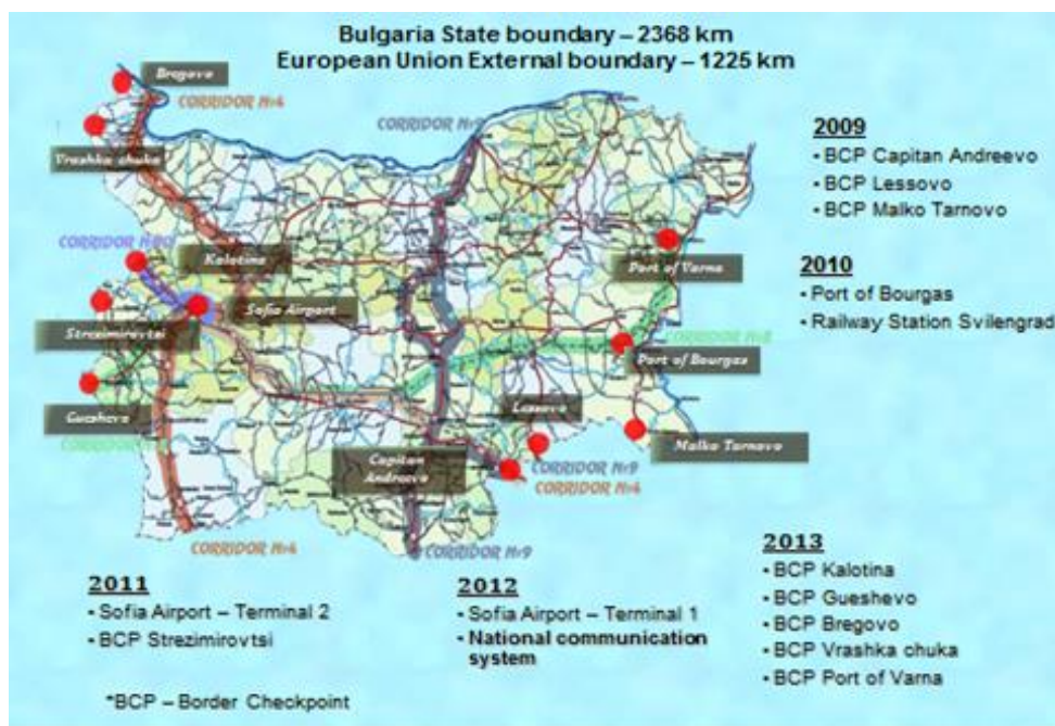
Fig 2 European Union external border – Bulgarian checkpoints
