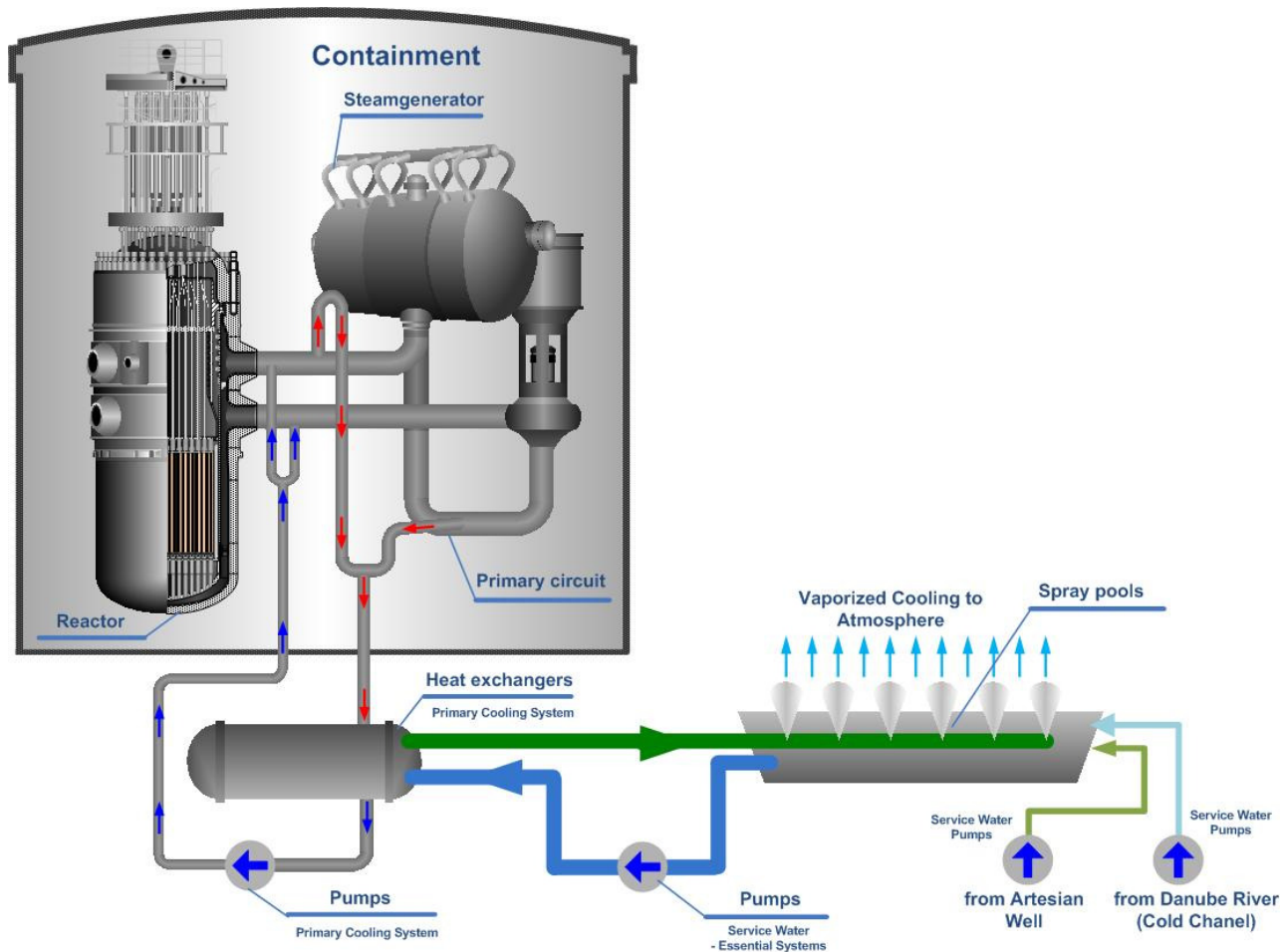
Figure 7. Water-water cooling
